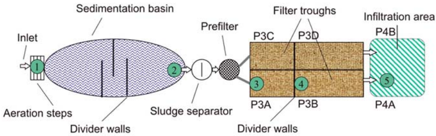
Figure 9.5. Pilot scale barrier (“natural treatment system”) in Ranstad. Circled numbers and P-labels (e.g. P3A) indicate sampling locations
