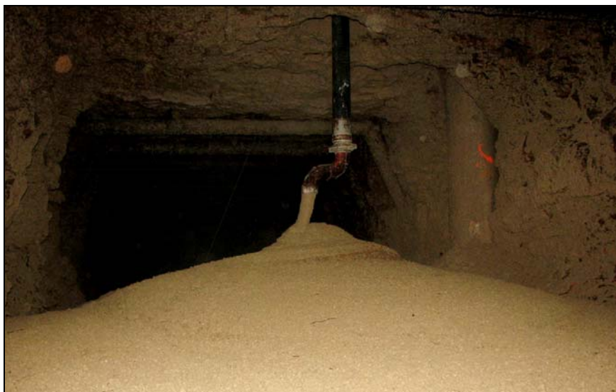
Figure 6.16. Hydraulic backfilling in an oil shale mine
