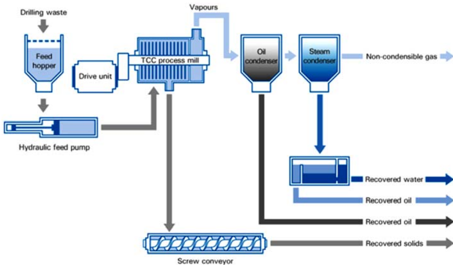
Figure 6.19. TCC Schematic
