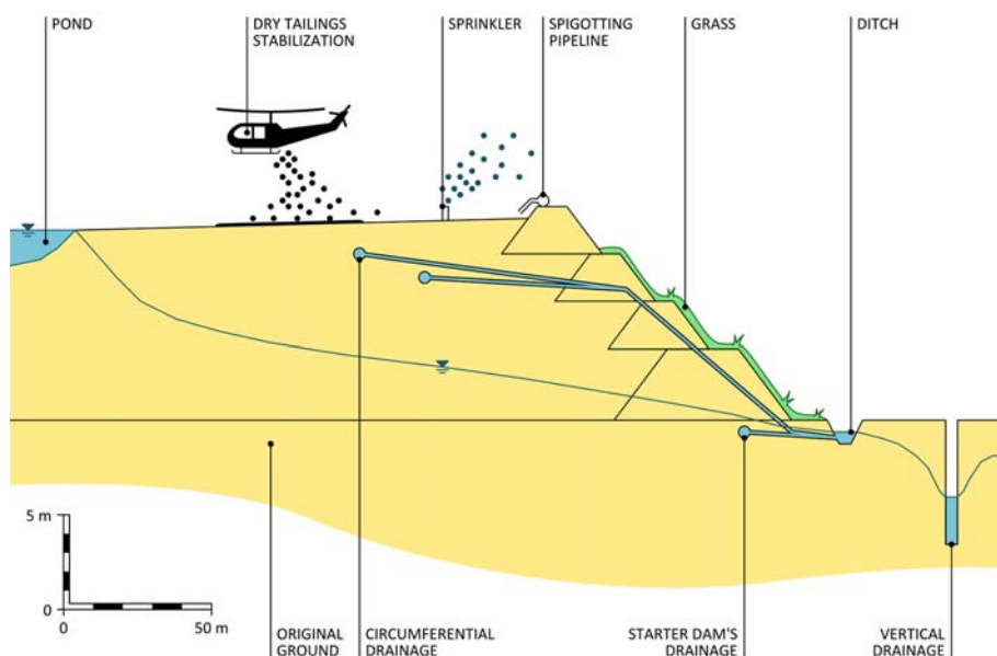
Figure 6.11. Actions reducing the Żelazny Most TSF environmental impact
