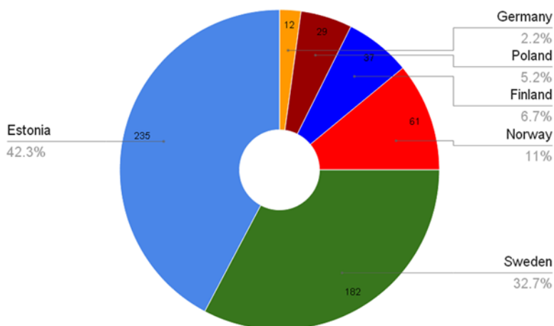
Figure 3.3. Database statistics
