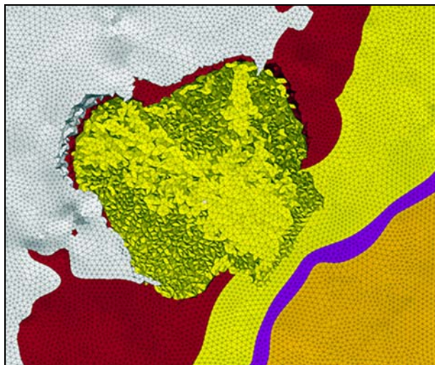
Figure 9.21. The final shape of the landslide obtained from 3D numerical calculations
