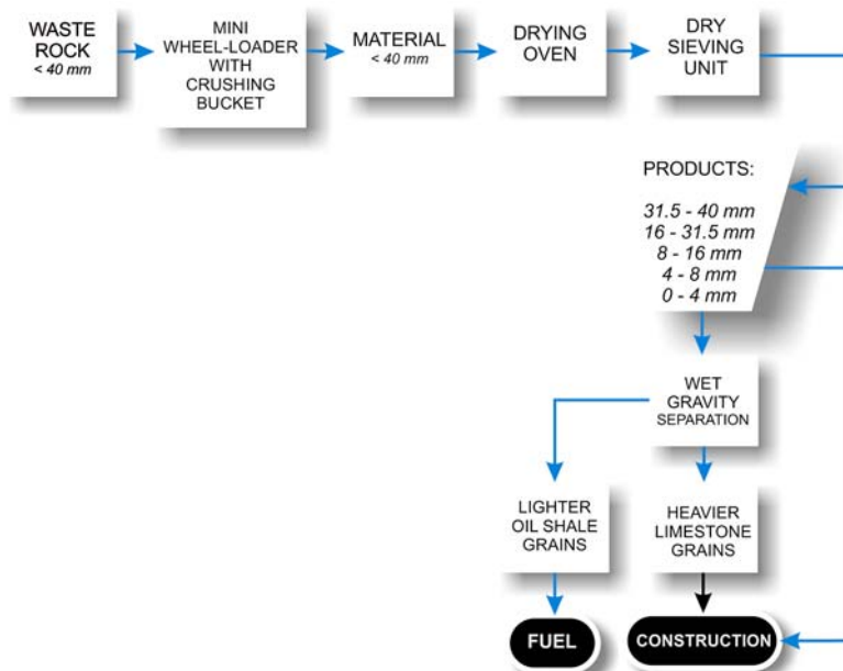
Figure 3.8. Scheme of mobile installation in the Tallinn University of Technology
