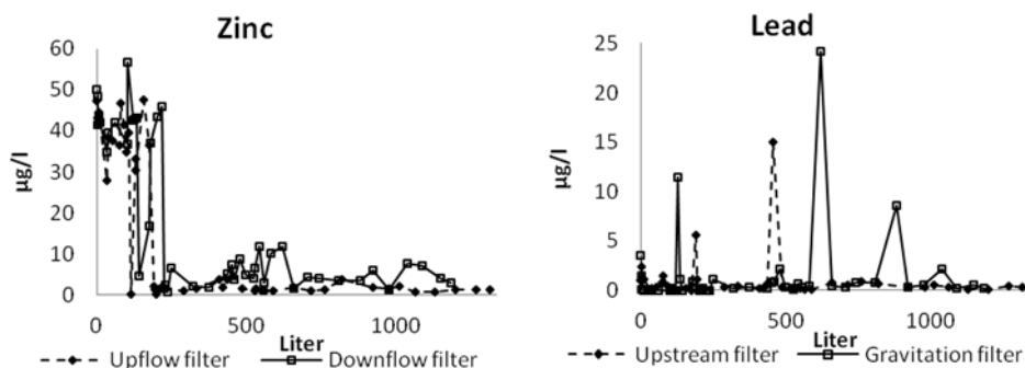
Figure 6.1. Zn in water filtered through the magnetite filter (Zn concentration in ingoing water: 690 µg/L) – left; Pb in water filtered through the magnetite filter (Pb concentration in ingoing water: 370 µg/L) – right
