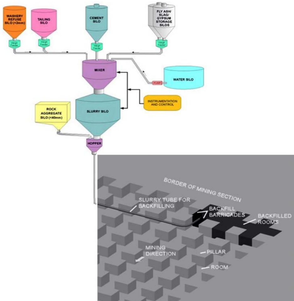
Figure 6.15. System of limestone wastes used in room backfilling in underground oil shale mines
