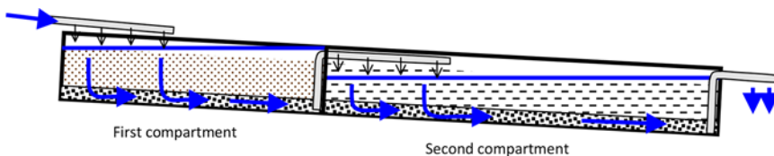
Figure 9.6. Cross-section of a filter trough containing two treatment compartments, in the final treatment step of the Ranstad barrier
