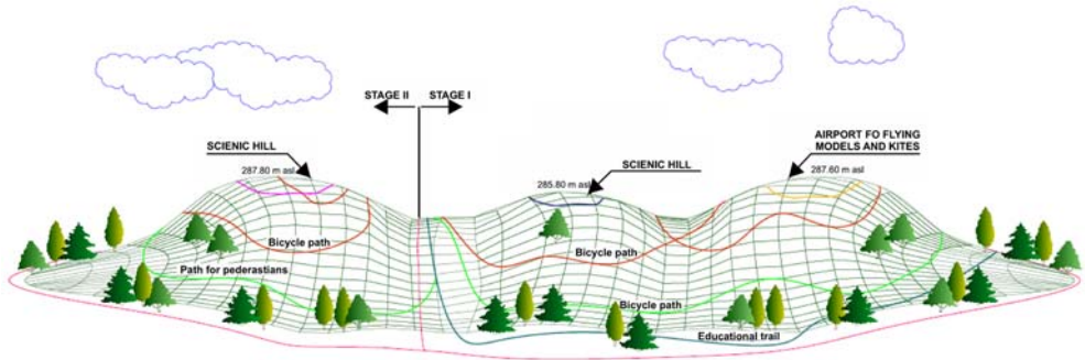
Figure 9.34. Three hills built with aggregates produced on the basis of waste rock and different binders at the Janina Hard Coal Mine area; Libiąż, Poland
